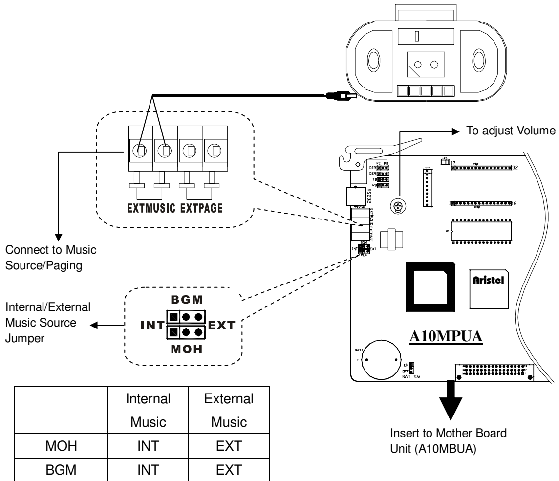
Chart 25: AV-48 External Music Source Installation
