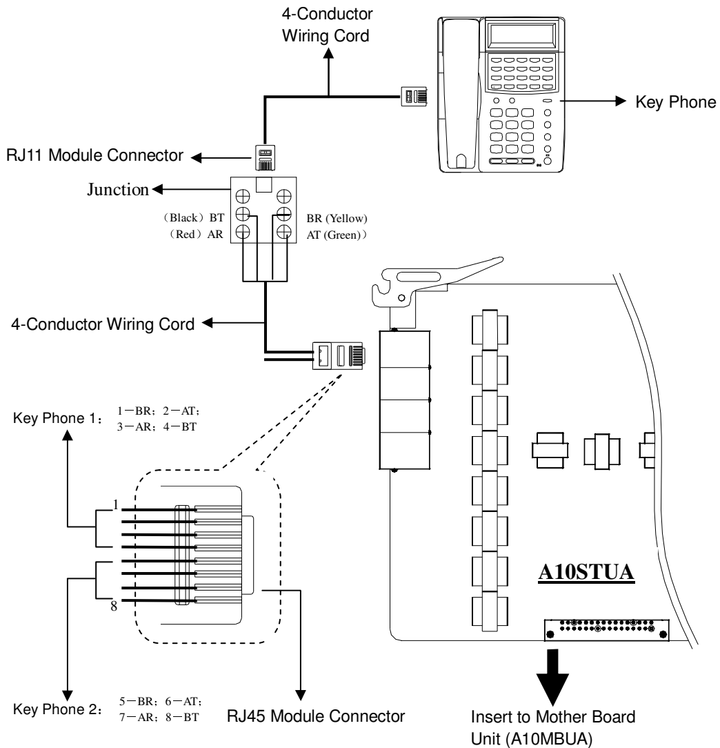
Chart 20: AV-48 Key Phone Station Wiring
