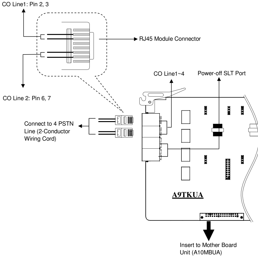
Chart 18: AV-48 CO Line Wiring
