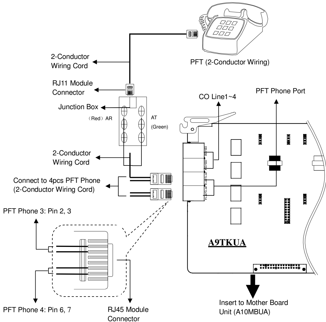
Chart 19: AV-48 Power Failure Transfer (PFT) Phone Wiring
