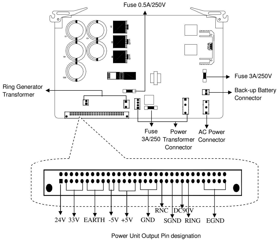
Chart 6: AV-48 Power Unit (A10PWUA)
