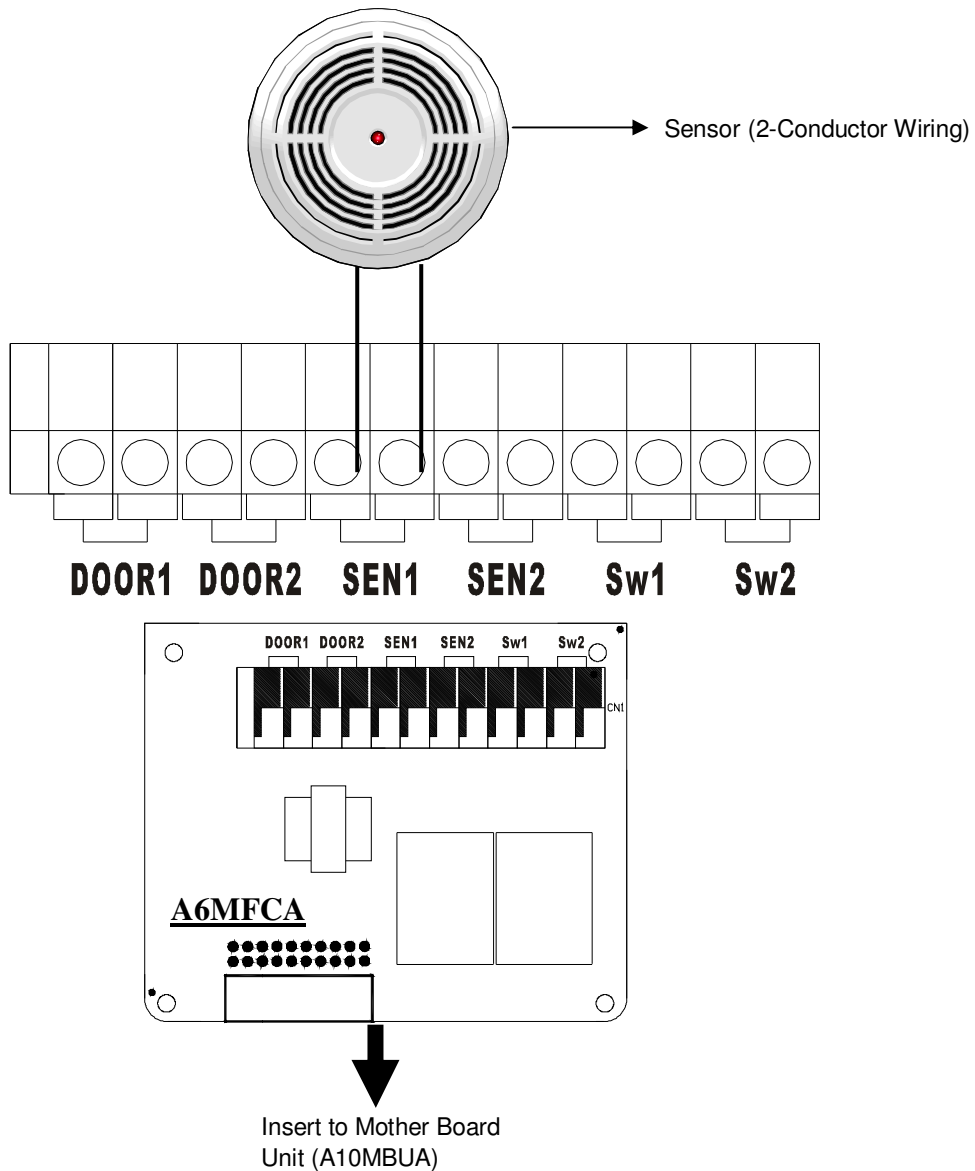
图 23: AV-48 Multi-function Sensor Installation
