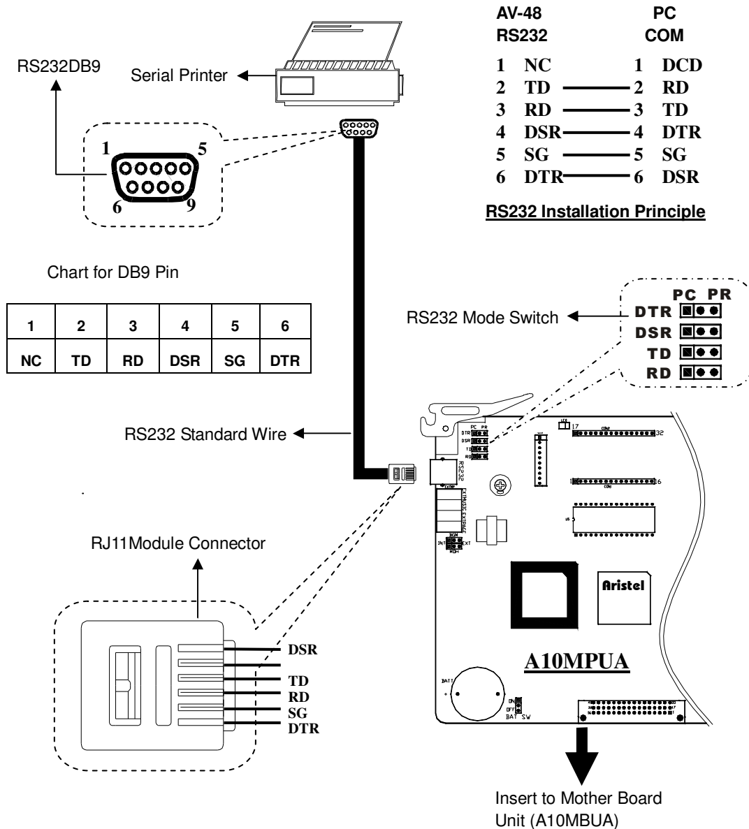
Chart 27: AV-48 RS232 (SMDR) Installation
