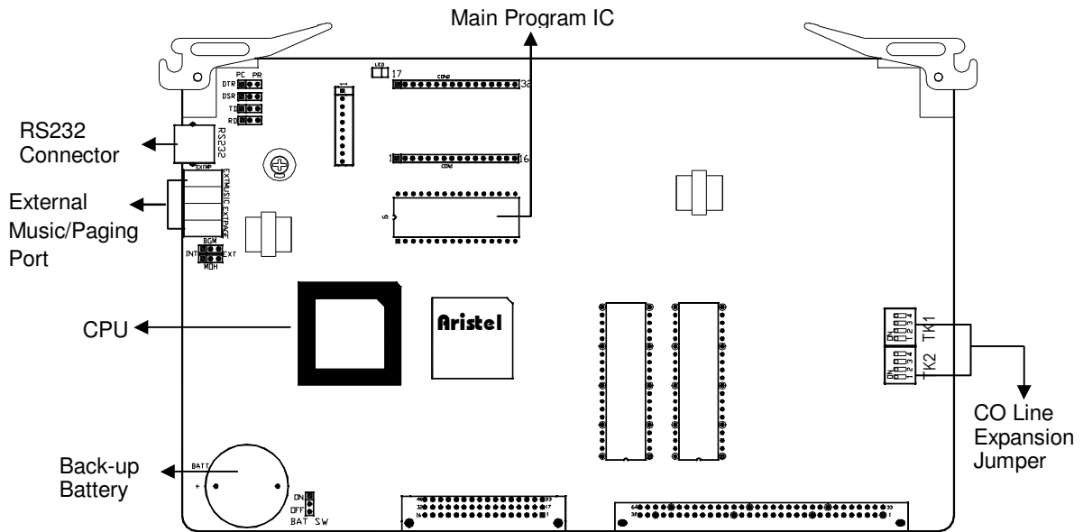
Chart 7: AV-48 Main Processing Unit (A10MPUA)
