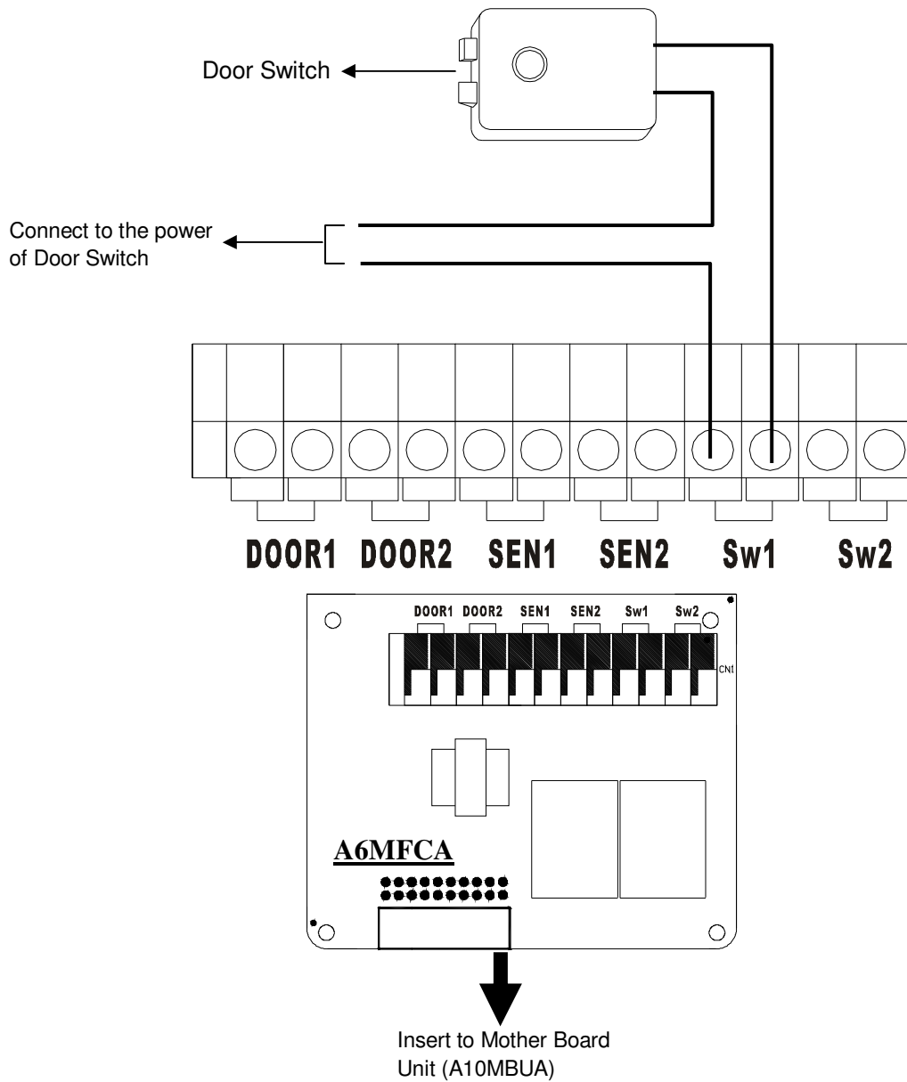
Chart 24: AV-48 Multi-function Relay—Door Switch Installation
