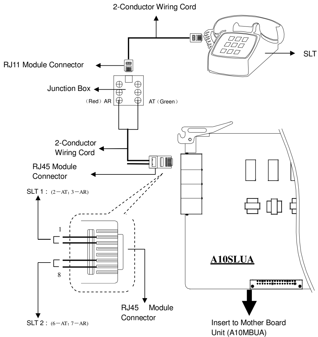
Chart 21: AV-48 Single Line Station Wiring
