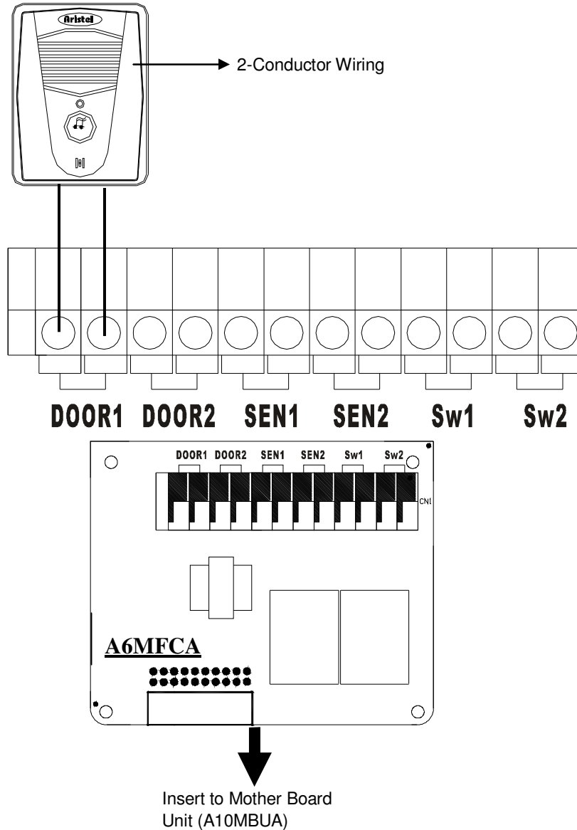
Chart 22: AV-48 Door Phone Installation
