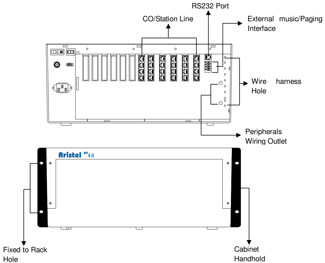
Chart 2: AV-48 built-in Standard Rack Layout
